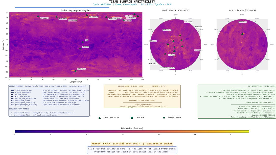
Figure 3.1: Present-epoch (Cassini era) posterior mean habitability map at 4490 m/px, rendered using the Bayesian temporal scaling formula (Section 2.6). Colour scale: 0.10 (dark red-orange; low) to 0.75 (bright yellow; near posterior upper bound). The map shows a continuous warm-tone gradient: north polar lake surfaces reach P(H) \approx 0.40 – 0.42 (orange-yellow), lake shore margins \approx 0.34 – 0.38 (orange), and equatorial organic terrain \approx 0.27 – 0.34 (dark orange-red). Selk crater is marked (star symbol) at 199^\circ\text{W} , 7^\circ\text{N} . Quantitative P(H) values in Sections 3.2.2–3.7.2 are Bayesian posterior means (Eq. 2.8), bounded in [0.150, 0.696] .
